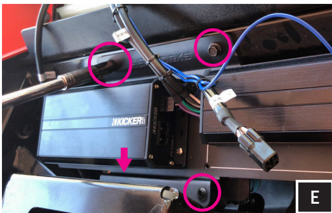
E. Secure the amp tray by using the two (2) 10mm factory bolts at the top, and two (2) T-30 torx bolts at the bottom mounting locations.
